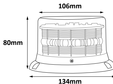
3-10012 angled rubber mount
